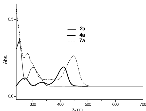
Figure 3. UV/Vis absorption spectra of compounds 2a , 4a and 7a in CH 3 CN.
