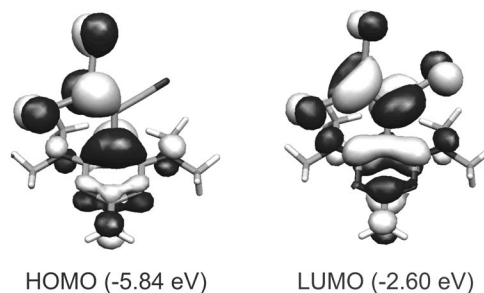
Figure 4. Electron density contours (0.03 eBohr −3 ) and energies (within parentheses) calculated for the HOMO and LUMO of 7a .
