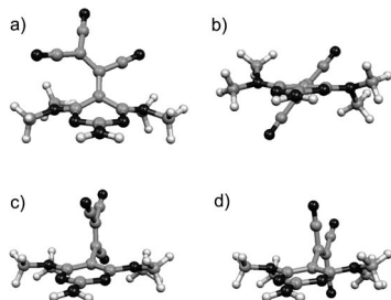
Figure 2. Minimum-energy conformations calculated for 7a at the B3LYP/6-31G** level.
