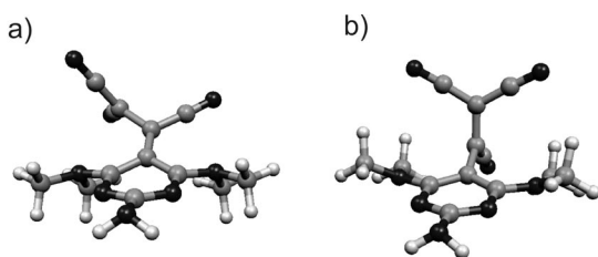
Figure 6. Minimum-energy conformations calculated for 7\text{a}^{2-} at the B3LYP/6-31G** level.
