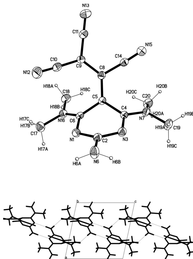
Figure 1. X-ray crystal structure of 7a .
